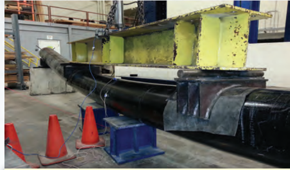
Full Section Testing of Concrete Filled Pile
