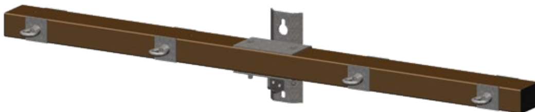
4 Phase Double Sided Deadend
